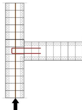
Figure 67 Etape 1
