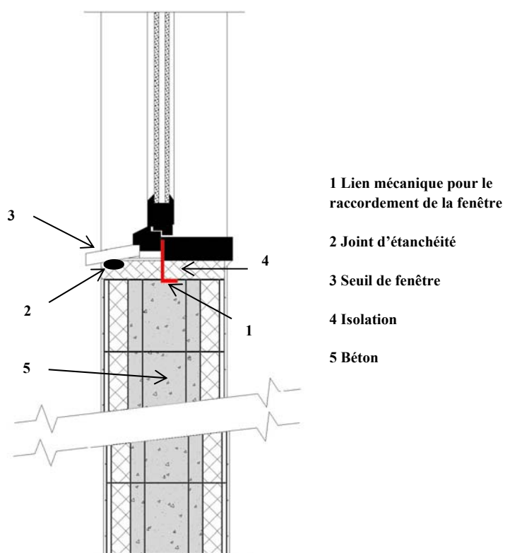
Figure 31 Coupe verticale
