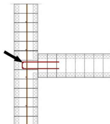
Figure 70 Etape 4
