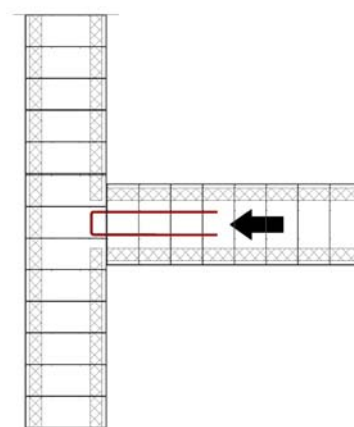
Figure 68 Etape 2
